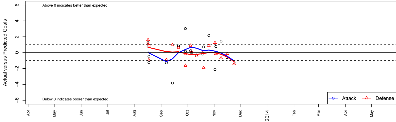
Laguna United Blue B02 Dots are actual minus expected GF (blue circles) and GA (red triangles). Blue line is smoothed change in attack strength. Red is smoothed change in defense strength.
